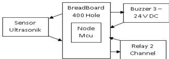
Gambar 1. Diagram Blok
